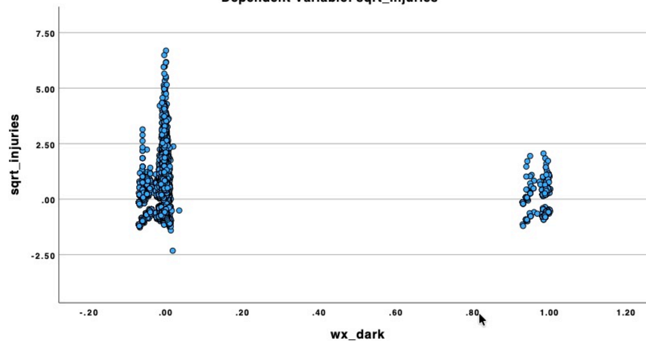
Partial Regression Plot Dependent Variable: sqrt_injuries
