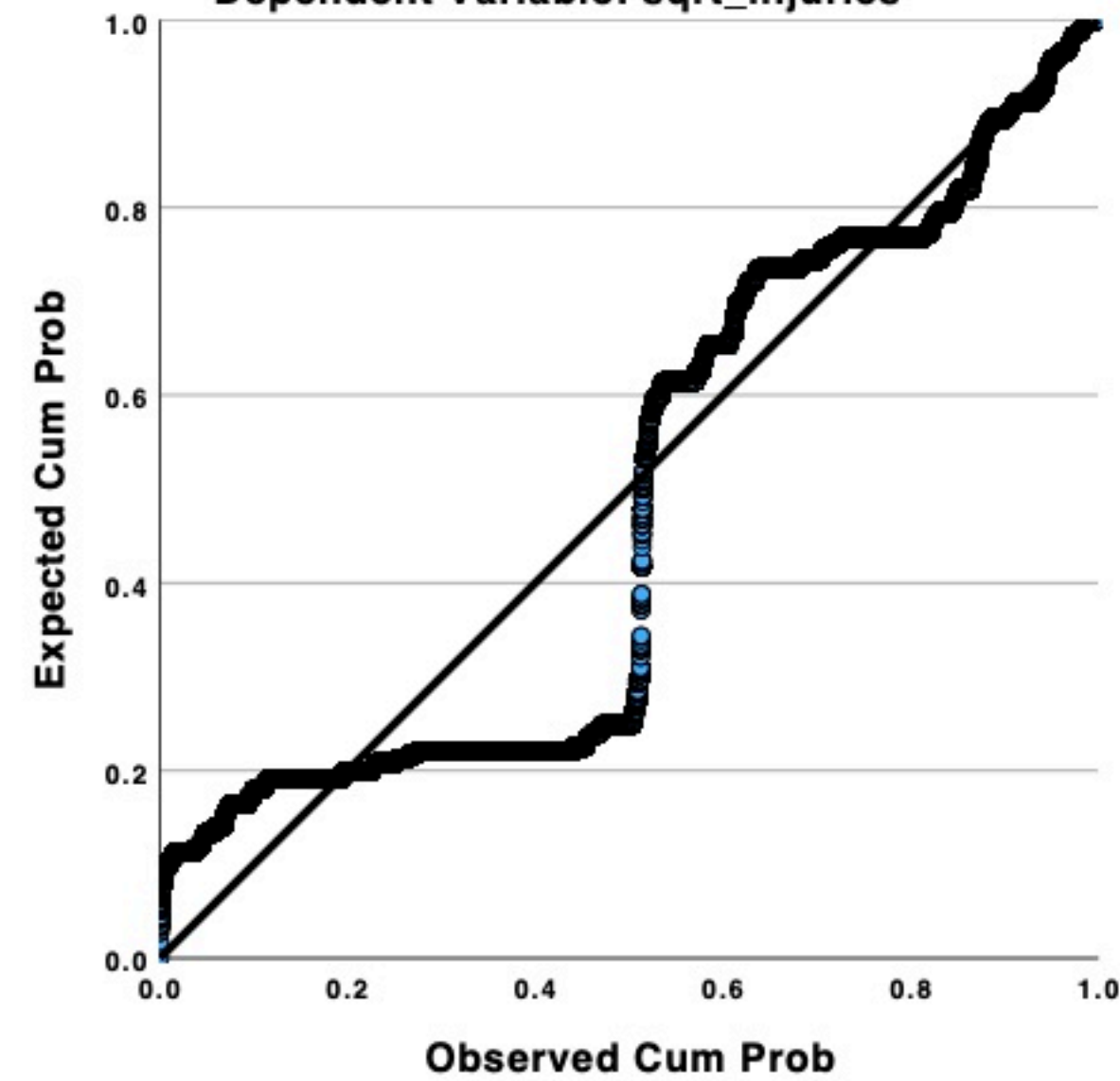
Normal P-P Plot of Regression Standardized Residual Dependent Variable: sqrt_injuries
